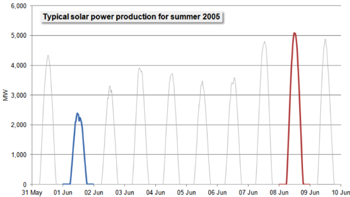
FIGURE 23A: EXAMPLE OF SUMMER PRODUCTION
