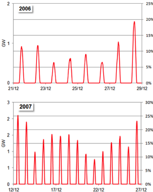
FIGURES 32A AND 32B: SOLAR POWER OUTPUT BELOW 10% AND 20% OF INSTALLED CAPACITY
