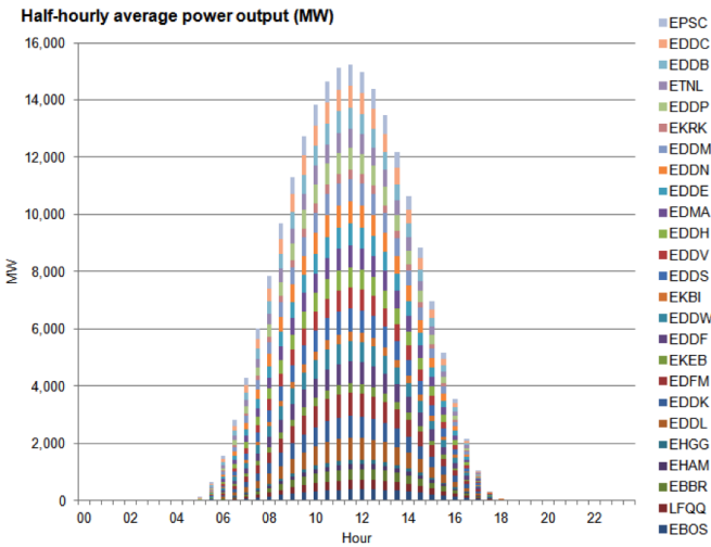
FIGURE A4: HOURLY POWER OUTPUT OF THE NORTHERN EUROPEAN SOLAR FLEET
