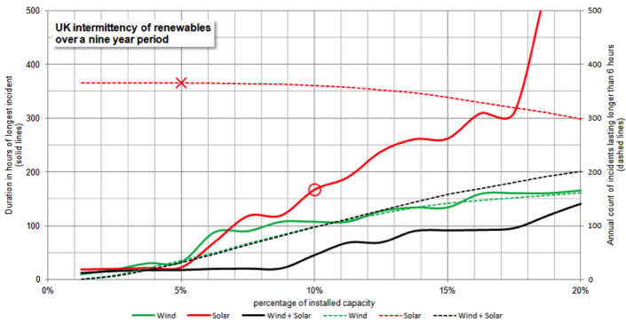
FIGURE 34: THE SCALE OF RENEWABLE INTERMITTENCY
