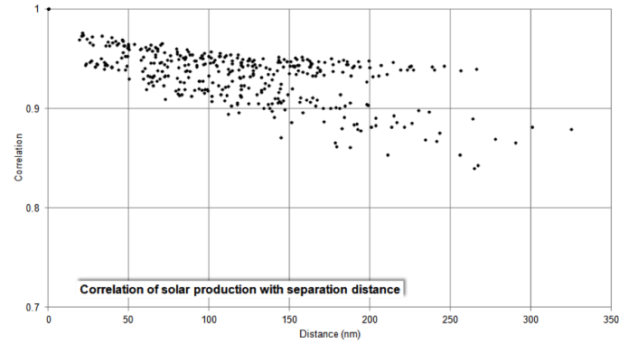
FIGURE 8: CORRELATION OF SOLAR PRODUCTION AT EACH SITE WITH ADJACENT SITES
