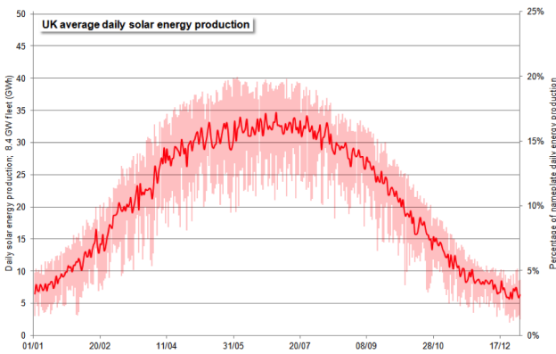
FIGURE 14: DAILY SOLAR ENERGY PRODUCTION THROUGHOUT THE YEAR *
