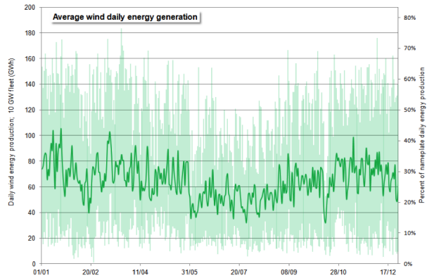
FIGURE 15: DAILY WIND ENERGY PRODUCTION THROUGHOUT THE YEAR*
