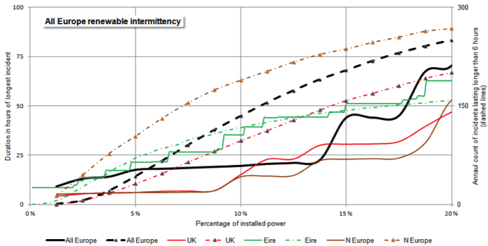
FIGURE 48: INTERMITTENCY DURATION AND INCIDENCE FOR THE WHOLE EUROPEAN GRID
