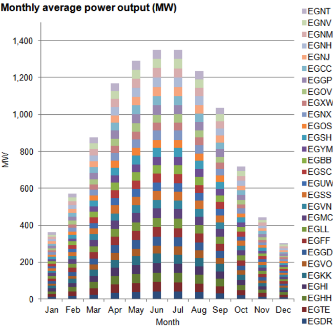
FIGURE 11: MONTHLY SOLAR FLEET OUTPUT - IN DECEMBER THE 8,400GW FLEET CAN ONLY DELIVER 300MW - WHEN NEW
